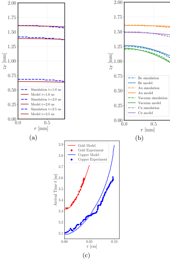
FIG. 3. (a) Model comparison with 2D diffusion simulation without hydrodynamics for the low-energy \text{SiO}_2 case [7], with Au coating, for 3 different times. (b) front curvature comparison with simulation between 4 different sleeves, Au, Cu, Be, and no sleeve (vacuum), showing the coating dependence. (c) Comparison with the French experiment of Courtois et al. [10], measuring front-arrival time versus radius for Au (1.2 mm) and Cu (2 mm) coatings.
