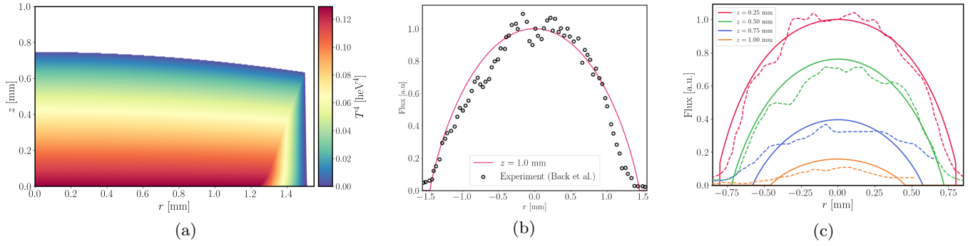
FIG. 4. Temperature reconstruction and flux curvature. (a) Two-dimensional T^4(r, z) profile obtained by the model at time 6 ns. (b) A cross section of the radial flux profile, compared with the Back et al. radial intensity data, at 1 mm inside the tube, 9.5 ns after the drive starts. (c) Additional experimental flux-curvature comparison for Ta 2 O 5 from Back et al. [8], taken at the temporal peak of the emitted x-ray signal (0.5 ns after breakout).
