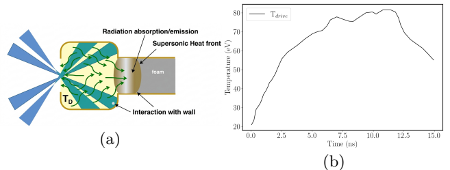
FIG. 1. (a) Experimental platform: laser beams enter the hohlraum through the LEH, generate x rays, and drive a Marshak wave in low-density foam targets of different lengths [9]. (b) Measured hohlraum drive temperature T_D(t) for the high-energy Back experiment [7].
